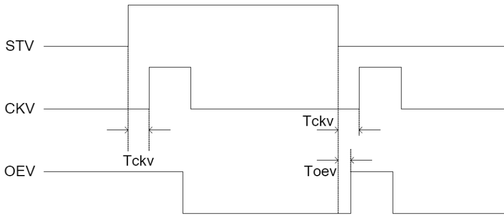
Figure: Vertical Timing Diagram DE
