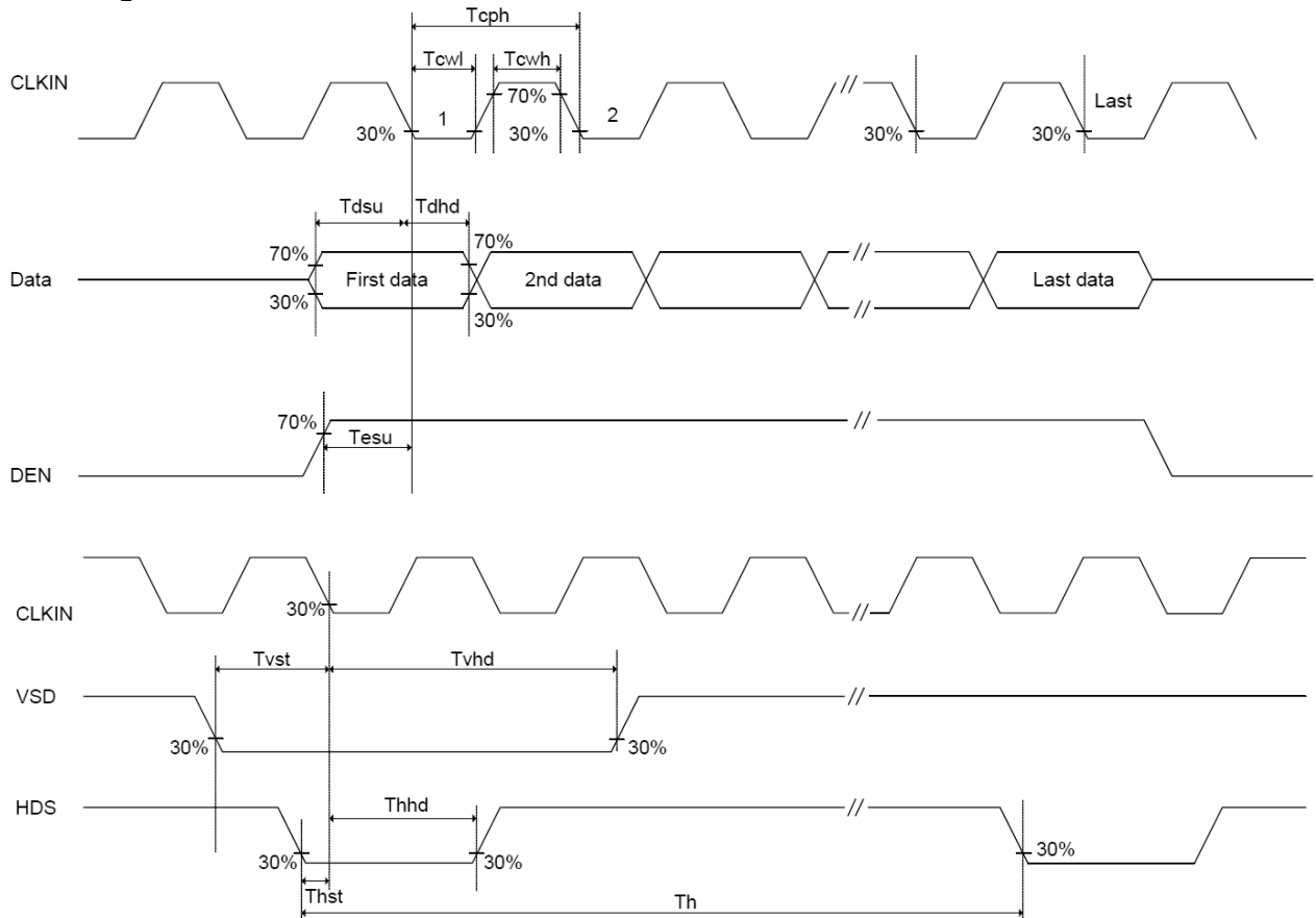
Figure: Input Clock and Data Timing Diagram
