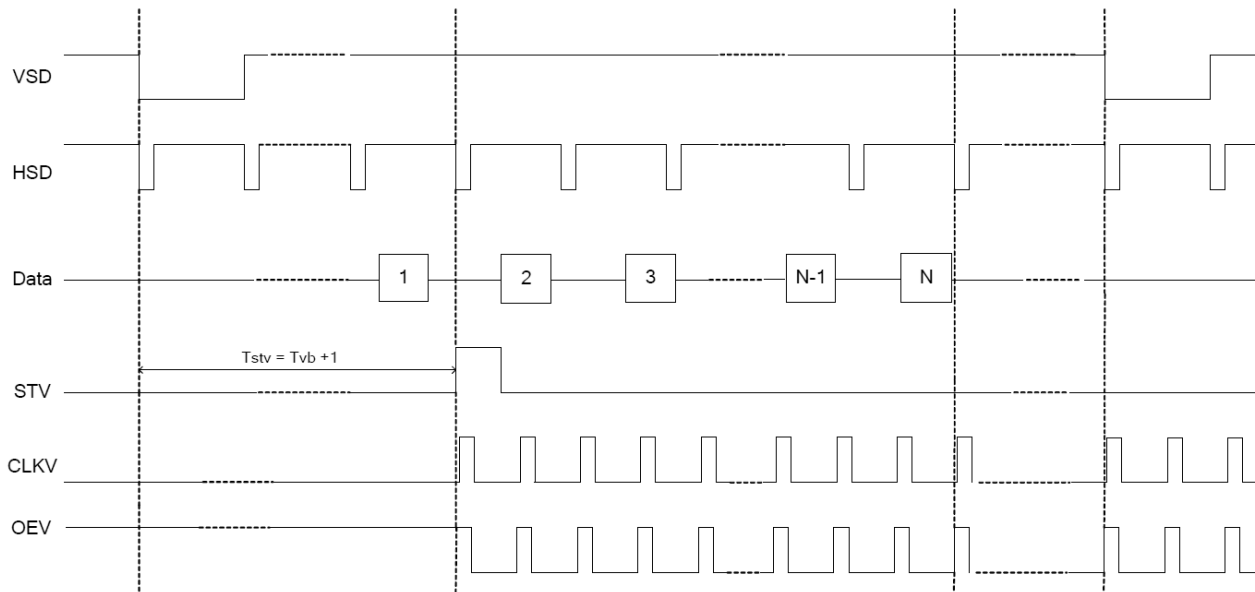
Figure: Vertical Timing Diagram HV
