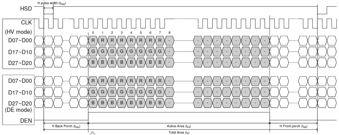
Figure: Horizontal input timing diagram
