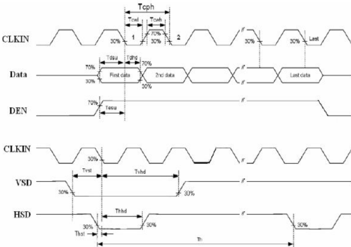
Input Clock and Data timing Diagram:
