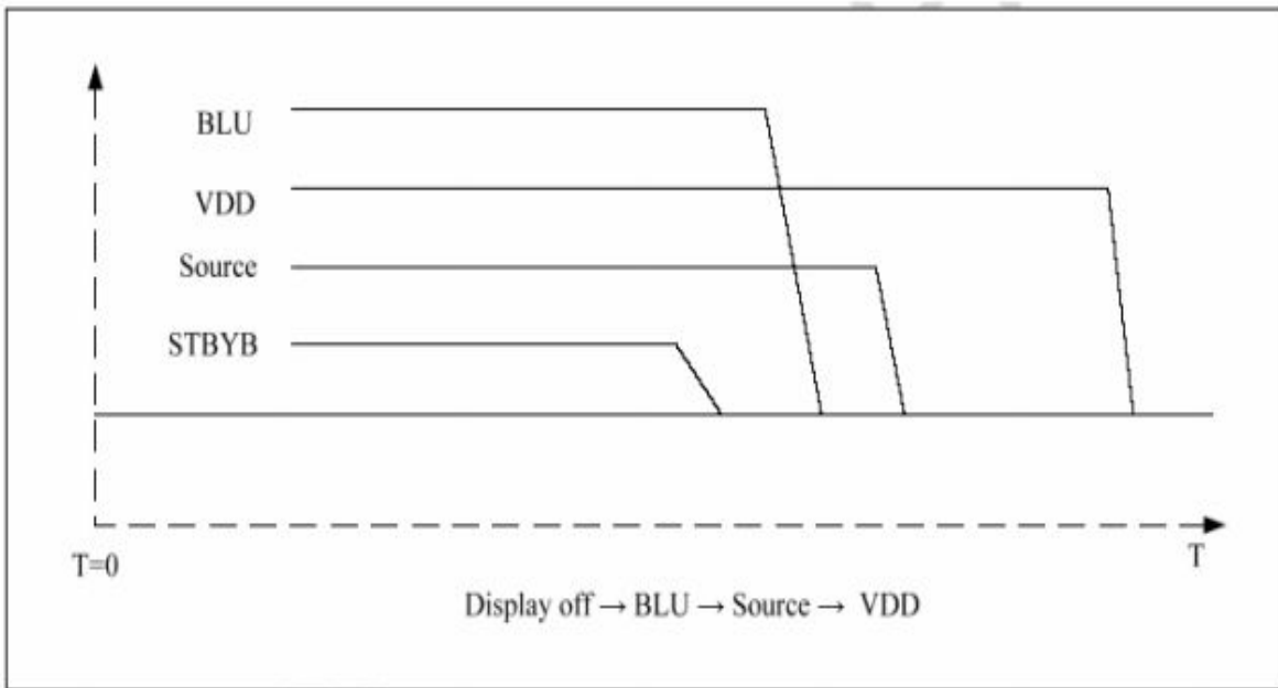
Power Off Sequence
