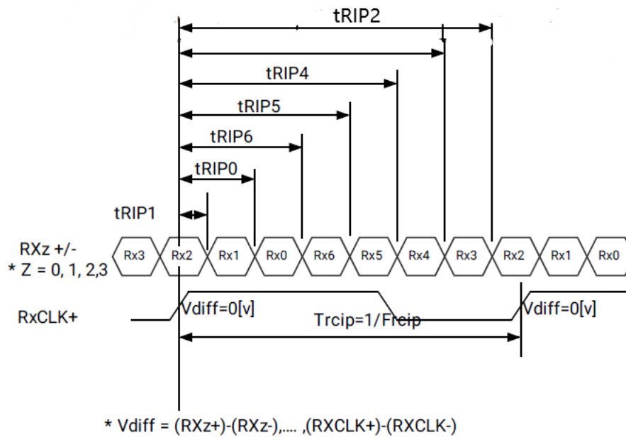
LVDS AC Timing Specification
