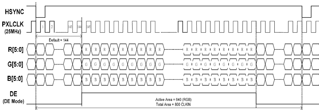
18 bit RGB mode for 640 x (RGB) x 480
