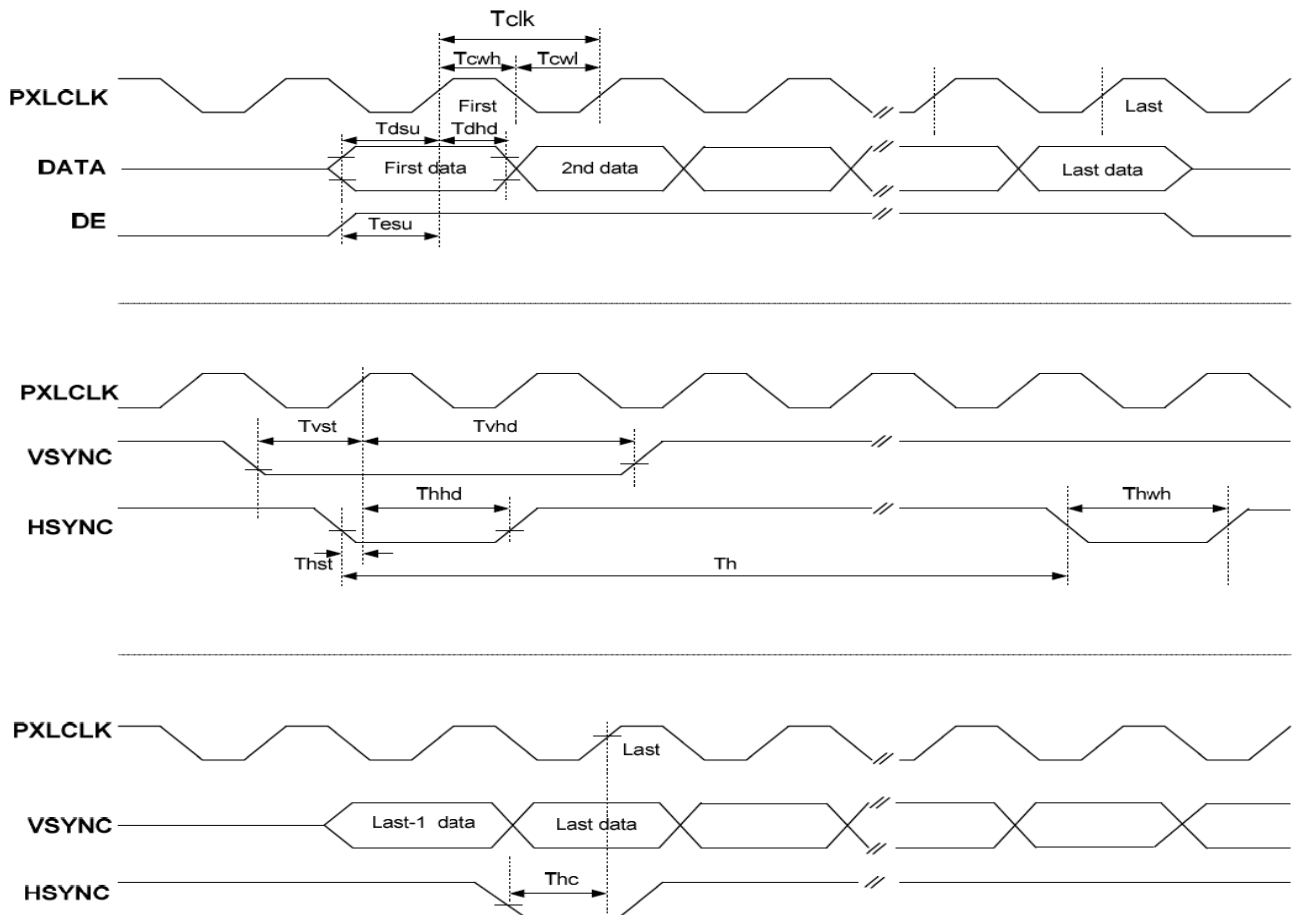
Clock and Data Input Timing Diagram
