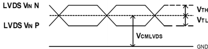
LVDS DC TIMING DIAGRAM
