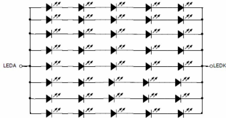
LED connection of Backlight
