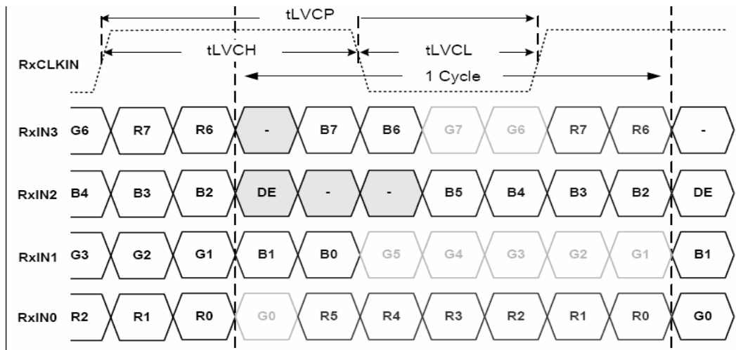
Input signal data timing
